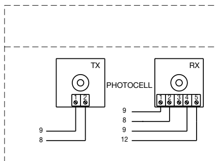
fig. 4c Photo with connection without phototest
