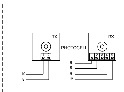
fig. 4a Photo with connection for phototest
