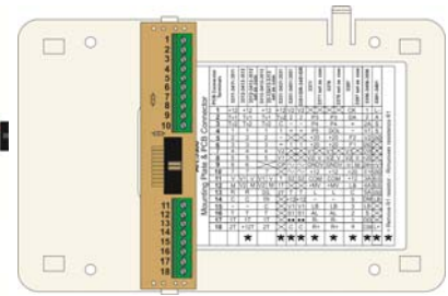
3980 (Back plate)
