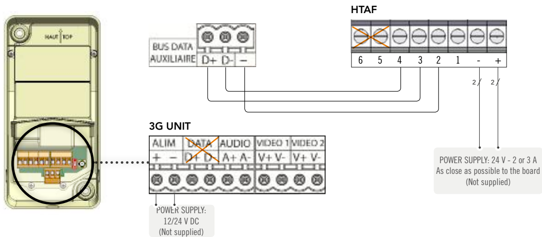
Diagram 1: simplified wiring
