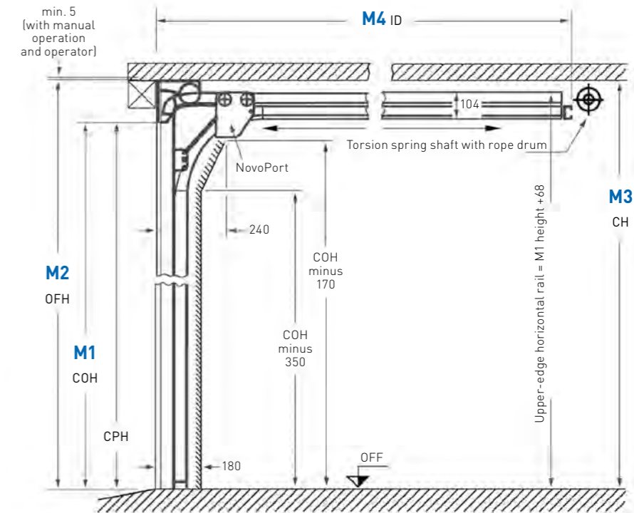
Fitting within the opening
