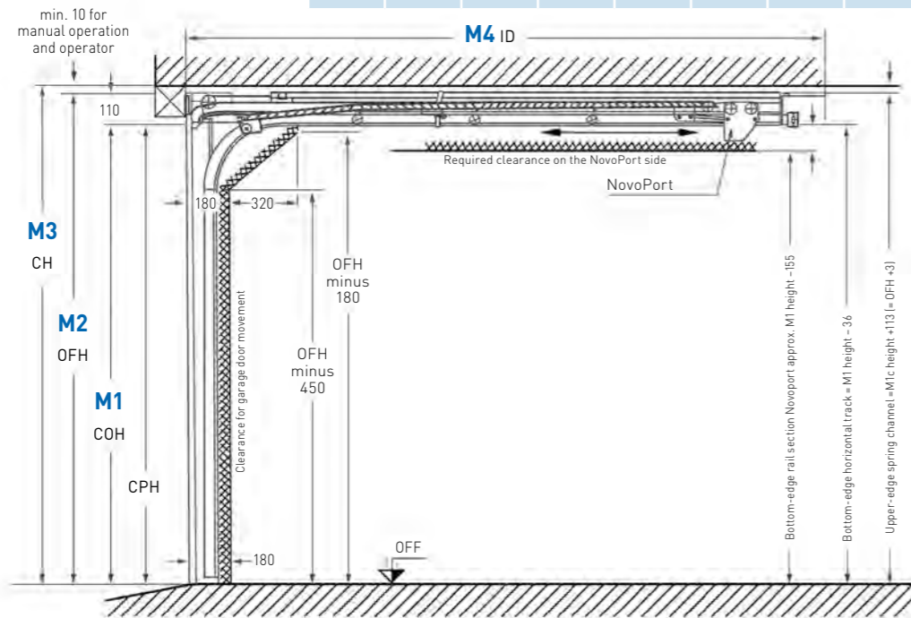
Fitting within the opening
