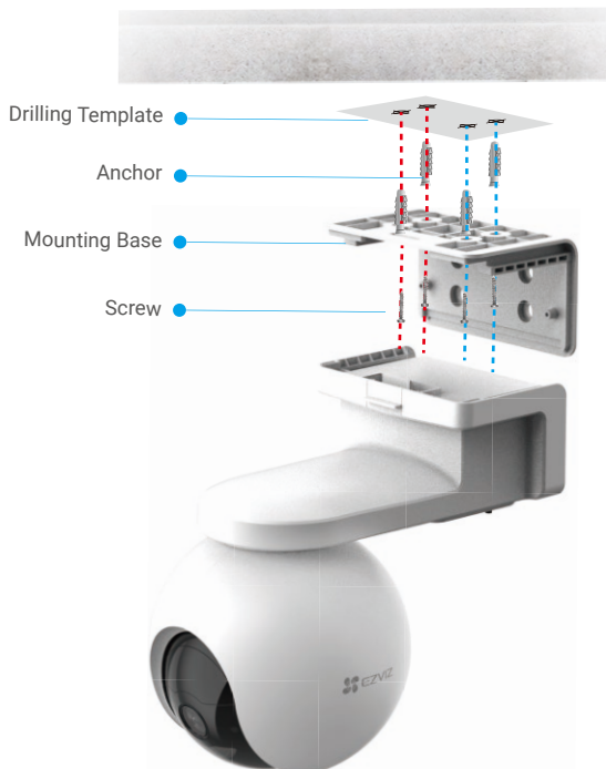
Fig. 1 Ceiling Mount
