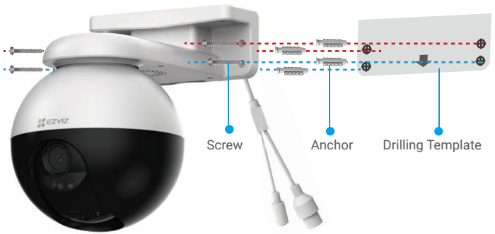
Fig. 2 Wall Mount
