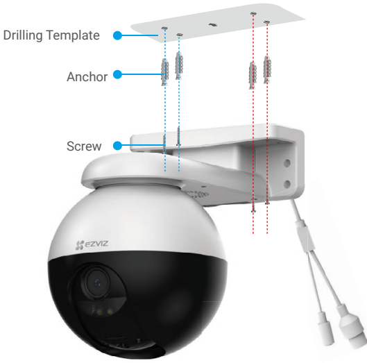
Fig. 1 Ceiling Mount
