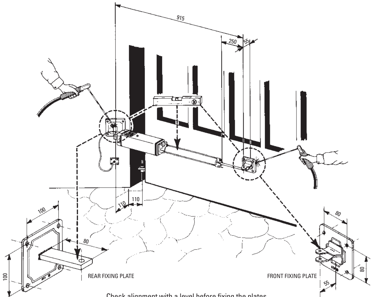
Check alignment with a level before fixing the plates Temporary set up for first tests
