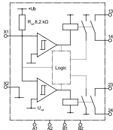
Simplified diagram SK 41
